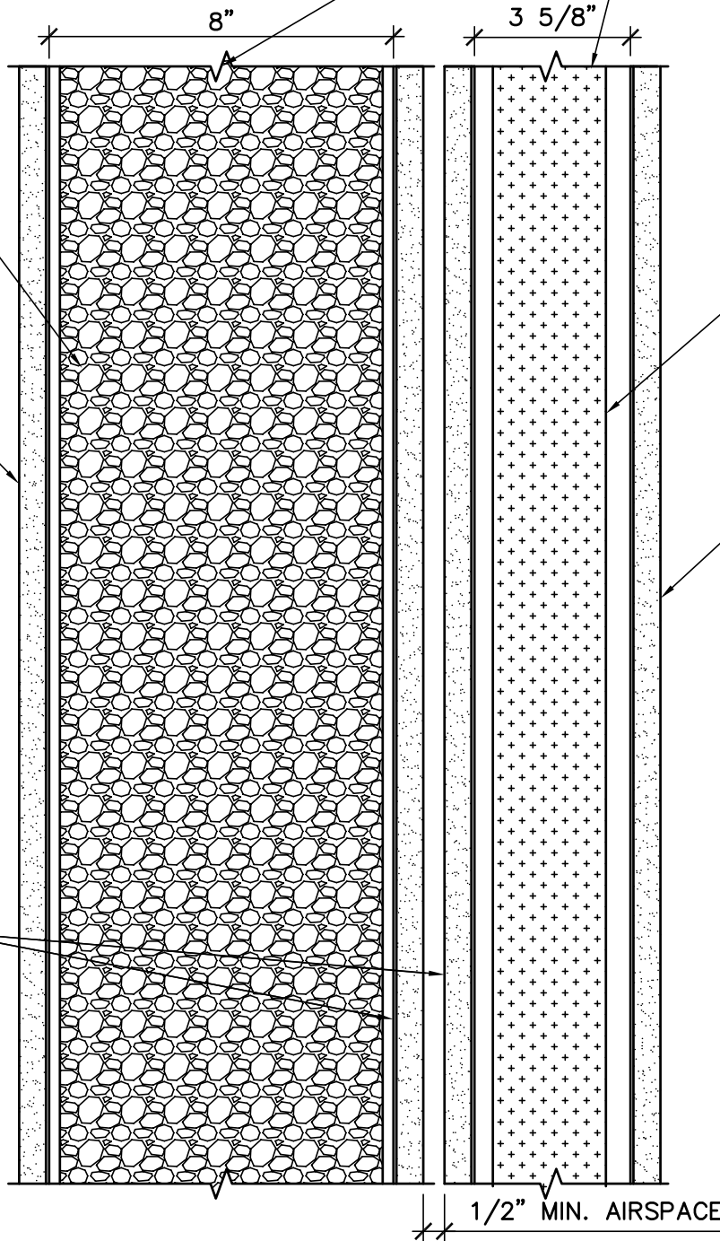
(A) TYPICAL LEVEL 10 BALLISTIC WALL ASSEMBLY
